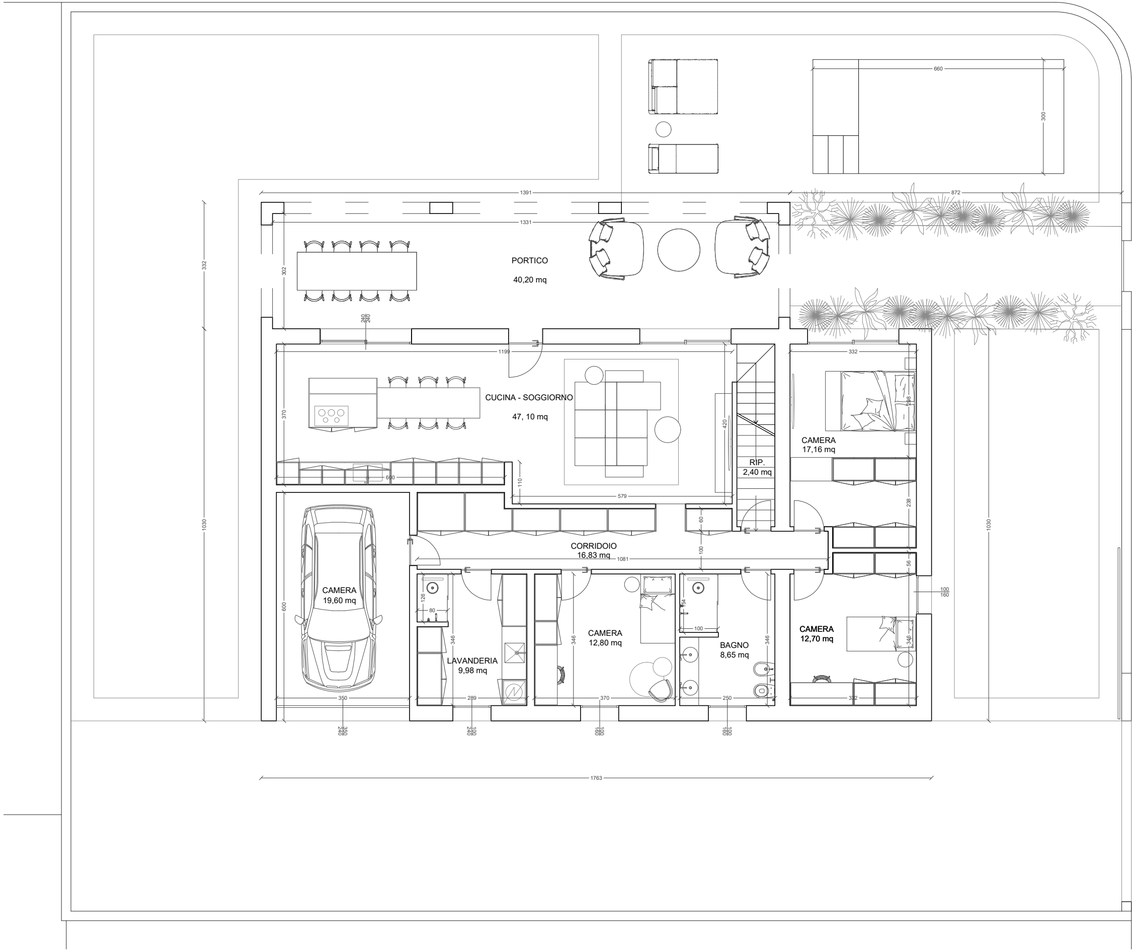
PLANIMETRIA PIANO TERRA
